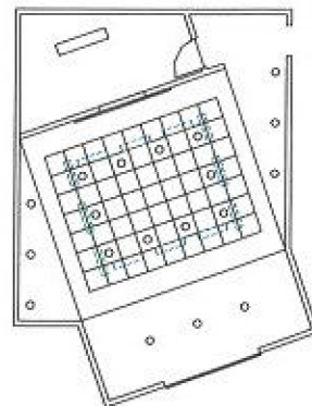
lighting plan
